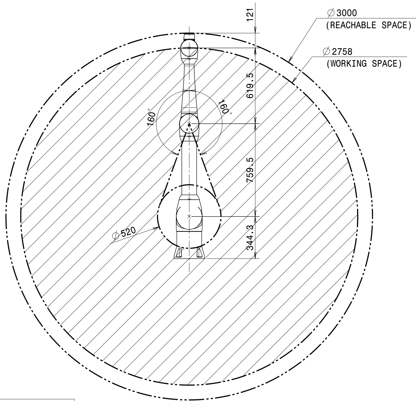
Front view (1:18)
