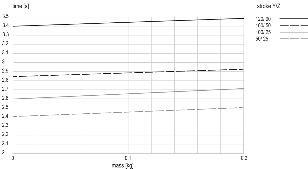
Cycle times EPS nano YZ for Pick & Place
