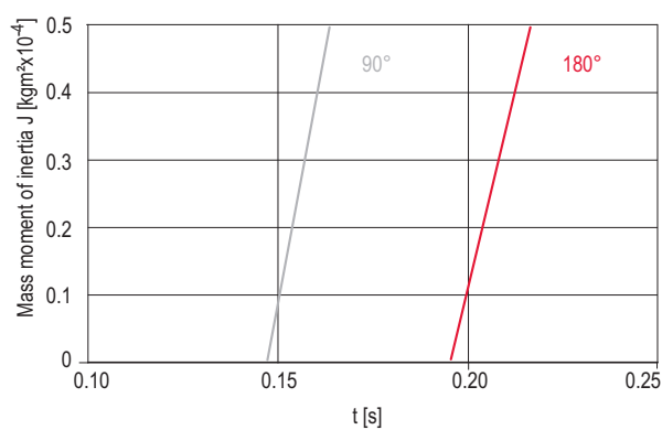
Rotation time
