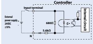
PNP specification
