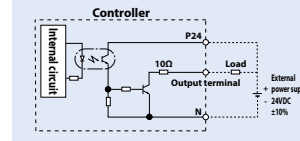
NPN specification
