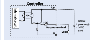
PNP specification
