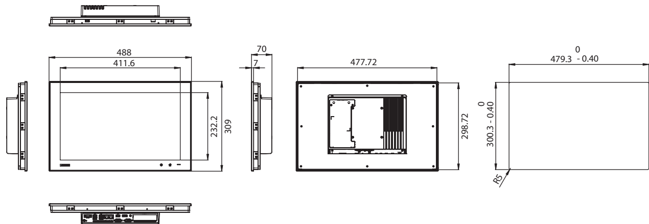
TPC-318WH Panel Cutout Dimensions: 479.3 x 300.3 mm (18.87 x 11.82 in)
