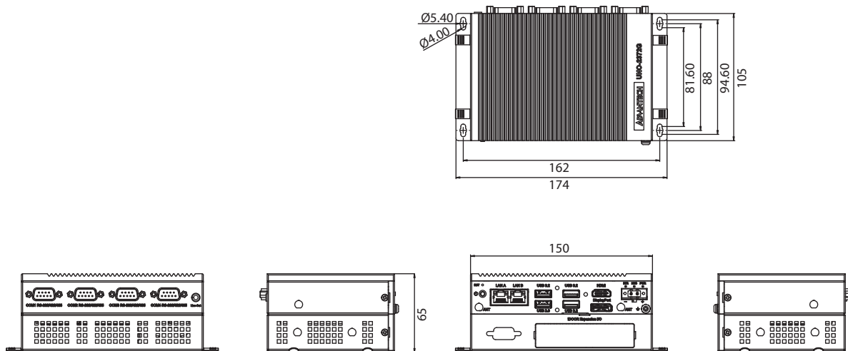
Double stack with UNO-2372G-EKCE
