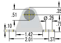
ME8 Bearing Shoe
