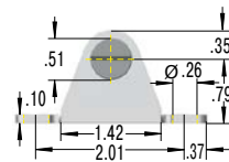
MA10 Bearing Shoe
