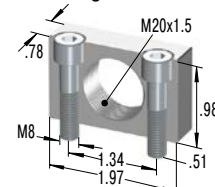
250-0436 Mounting Block
