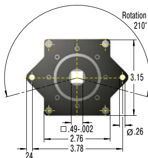
Keyed output shaft shown in mid-travel position
