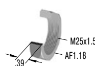
250-0443 Locknut
