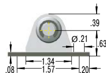
NG8 Angle Bracket
