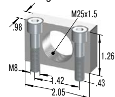
250-0436 Mounting Block
