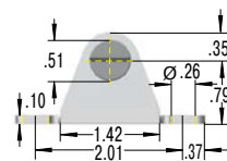
ME10 Bearing Shoe
