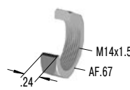
250-0441 Locknut
