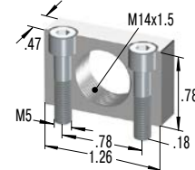
250-0434 Mounting Block
