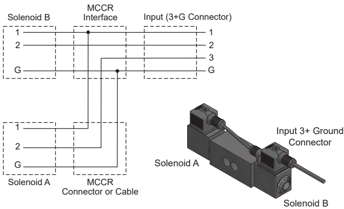
Separate Control Circuit Type #1 and Circuit Type #2
