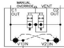
Model Types 60 & 61 Schematic
