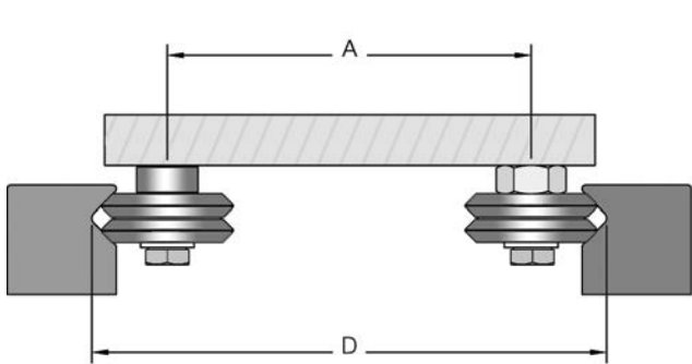
FIG. 3 EXTERIOR MOUNTING
