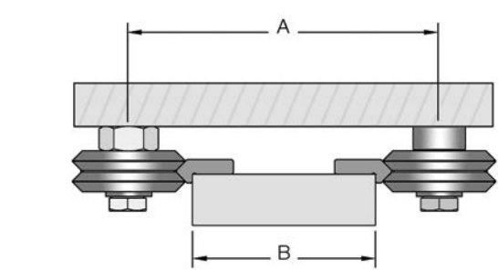
FIG. 1 INBOARD MOUNTING
