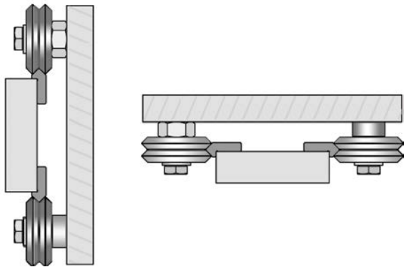
MOUNTING ORIENTATIONS
