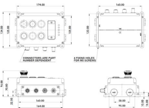
NET-BOX DIECAST
